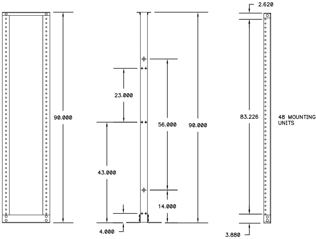
FRONT VIEW UNIVERSAL RACK
