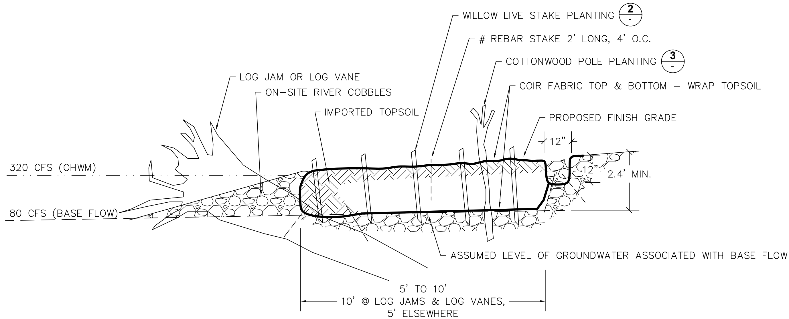
COIR FABRIC, TOPSOIL & PLANTING TYPICAL SECTION
