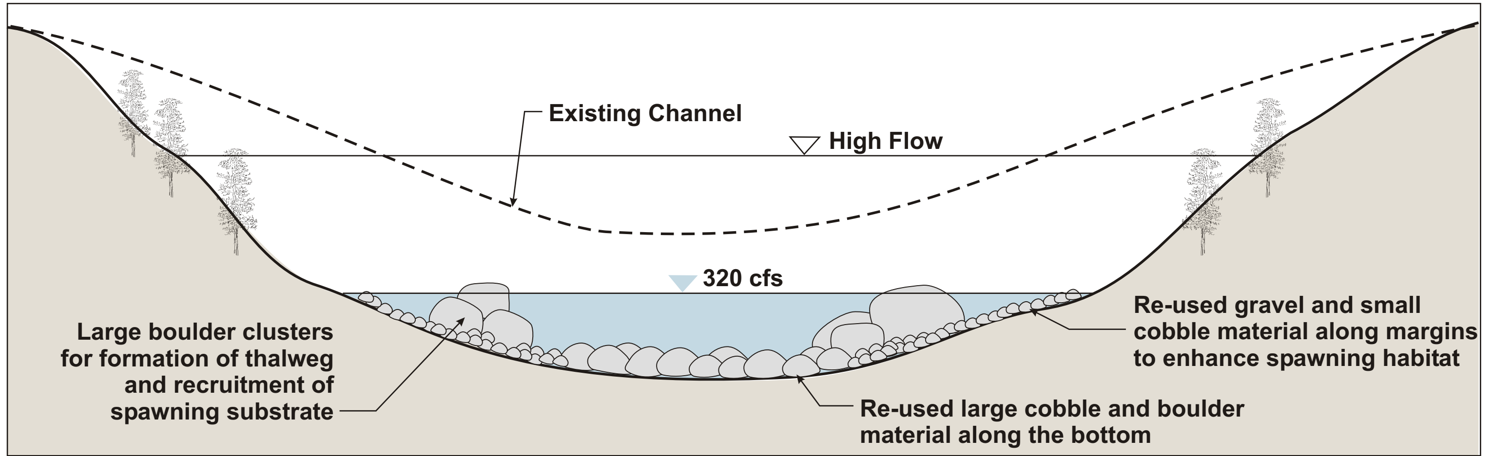
Option 2 - Single Main Channel Cross Section A-A'
