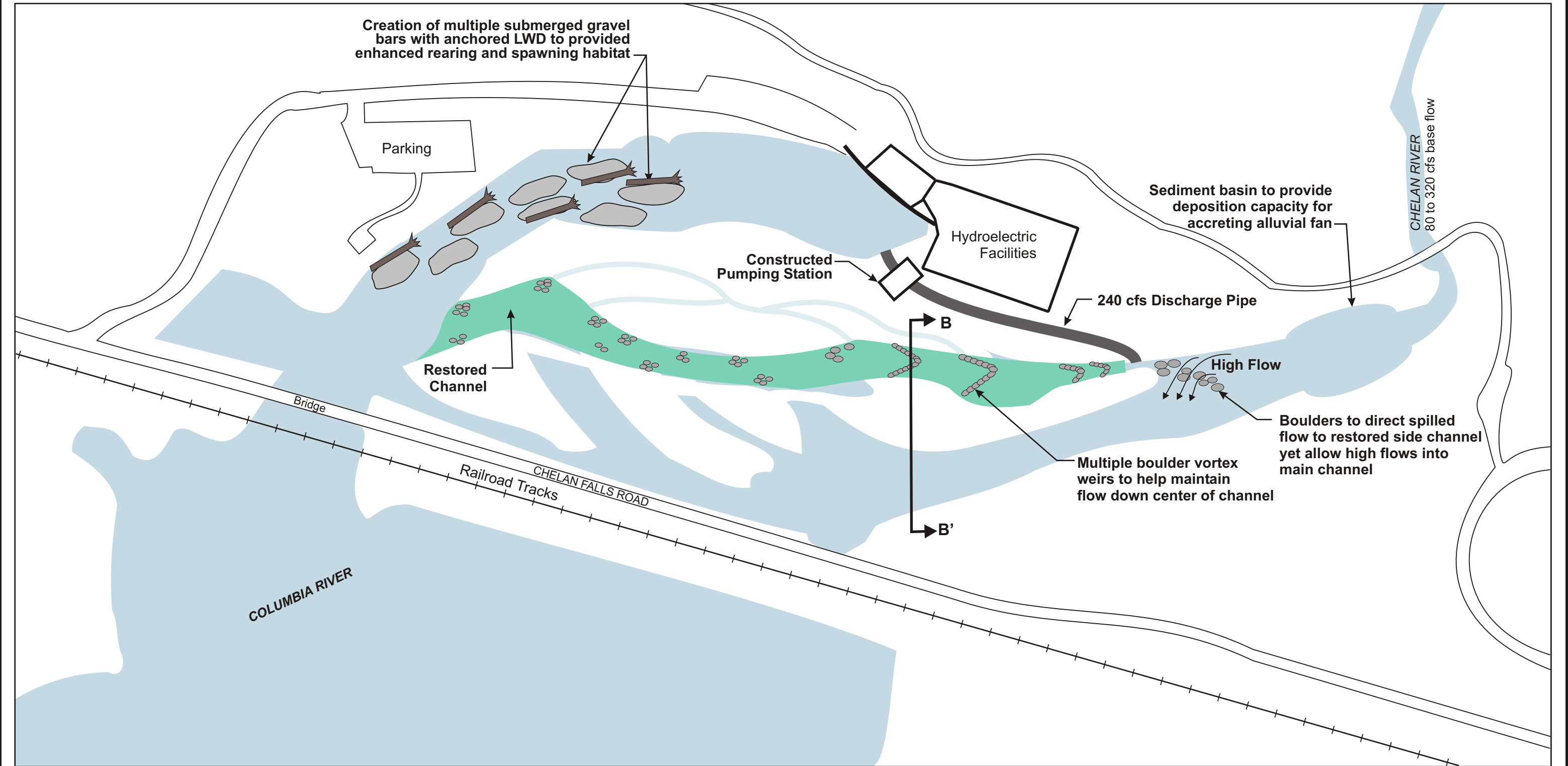
Option 1 - Floodplain "Side Channel" Plan View
