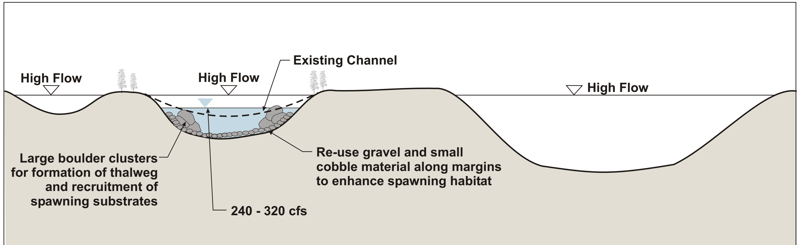
Option 1 - Floodplain "Side Channel" Cross Section B-B'
