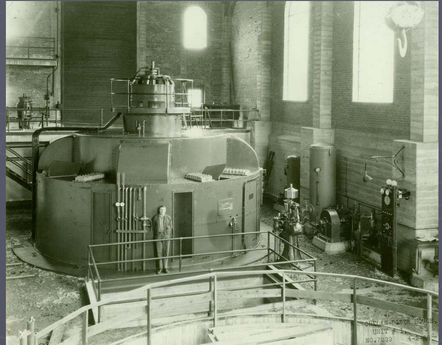
Original Generating Unit 1 - April 2, 1928
