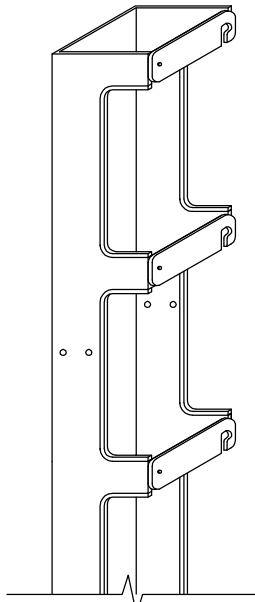
CABLE SECTION 6"W X 6.36"D X 7'6"H
