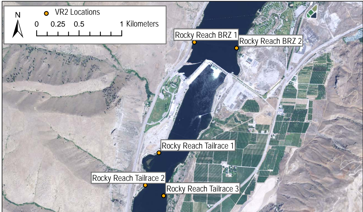
Figure C - 6. Locations of Vemco VR2W receivers deployed comprising the Rocky Reach BRZ array (RKM 763) and the Rocky Reach Tailrace array (RKM 761-762).
