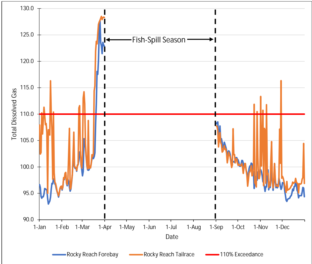
Figure 3-1. Daily maximum TDG reading from each FMS
