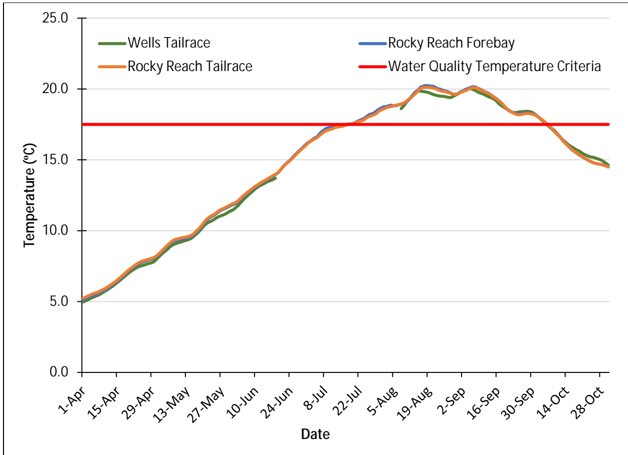
Figure 3-2. 7-DADMax Temperatures in the Wells tailrace, Rocky Reach forebay, and Rocky Reach tailrace
