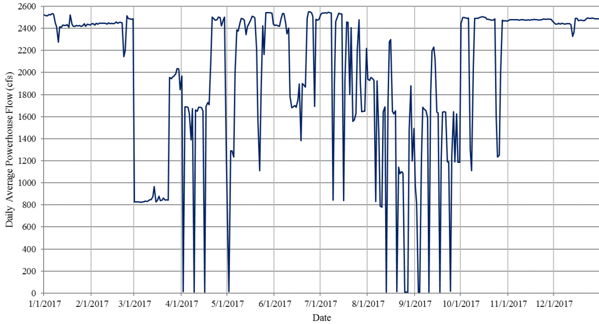
Figure 3-1. Chelan Powerhouse Daily Average Flows, 2017.
